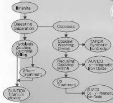
Chart of Processing Waste Acid Resource
